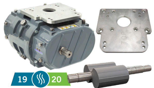
RS Advanced Technology patent pending coating on rotor lobes for reduced slip and optional lightweight aluminum adaptor plate displayed with blower.
